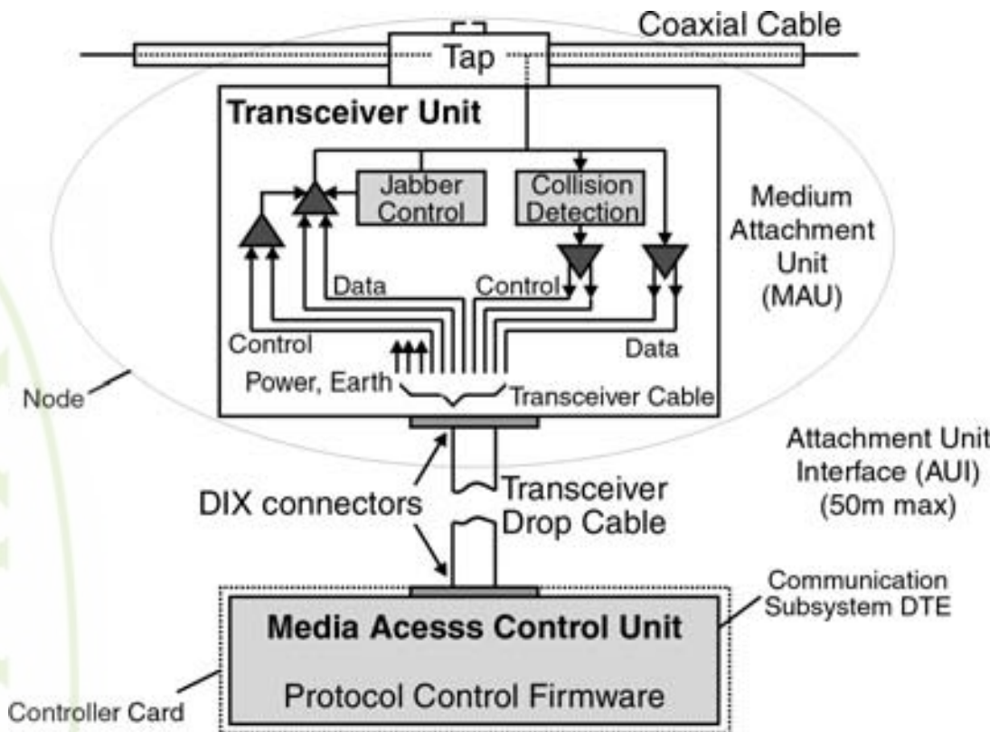
Figure 2.6 10BASE-5 Hardware Components
