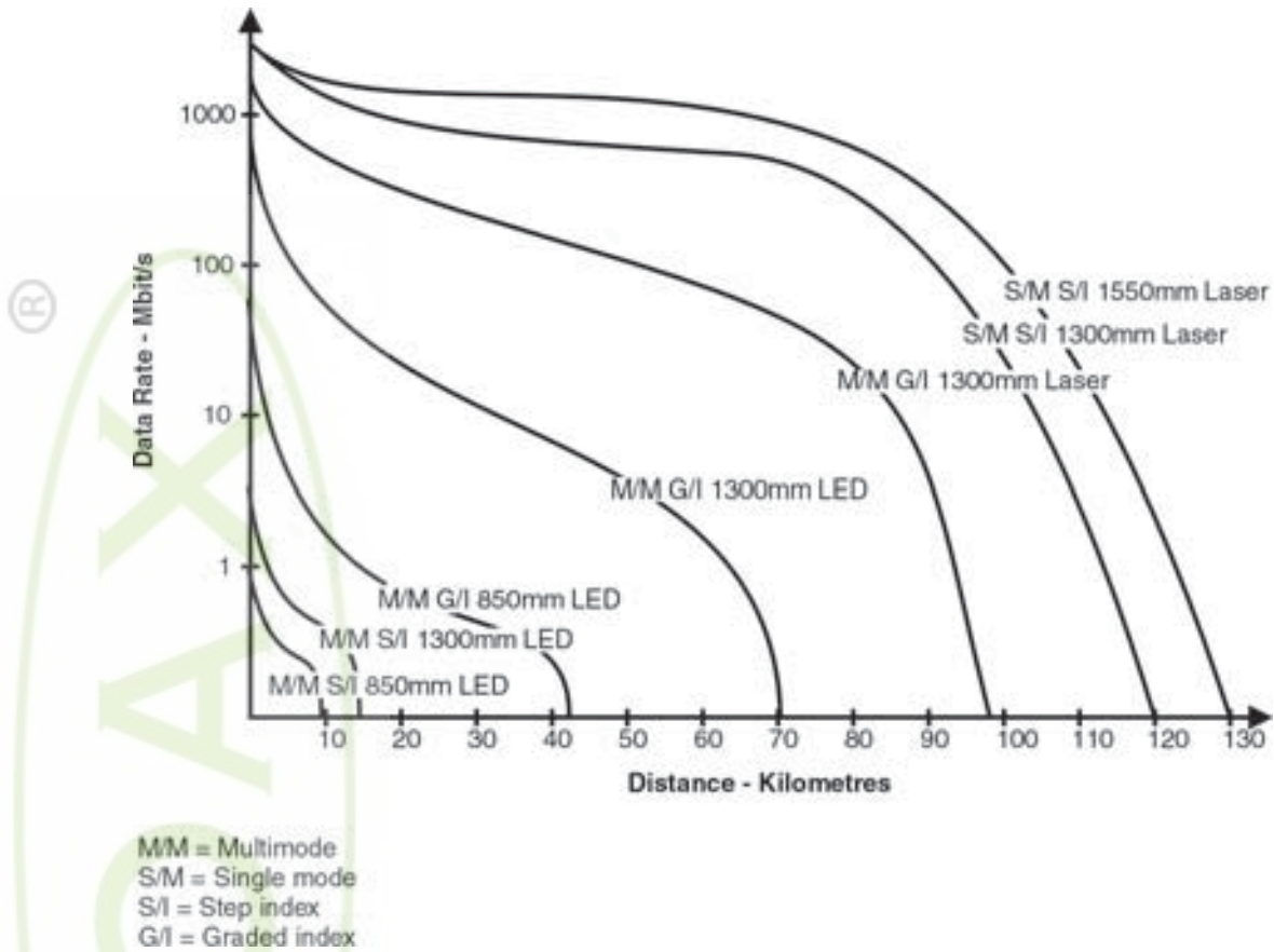
Figure 3.9 Comparison of Data Rate, Distance and Fiber Type
