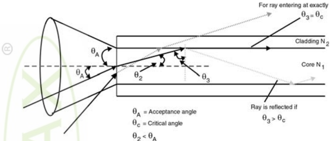
Figure 3.7 Cone of Acceptance of an Optic Fiber
