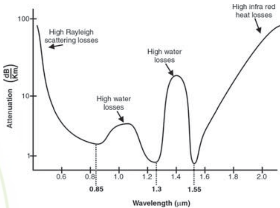
Figure 3.5 Typical Attenuation Responses for a Fiber
