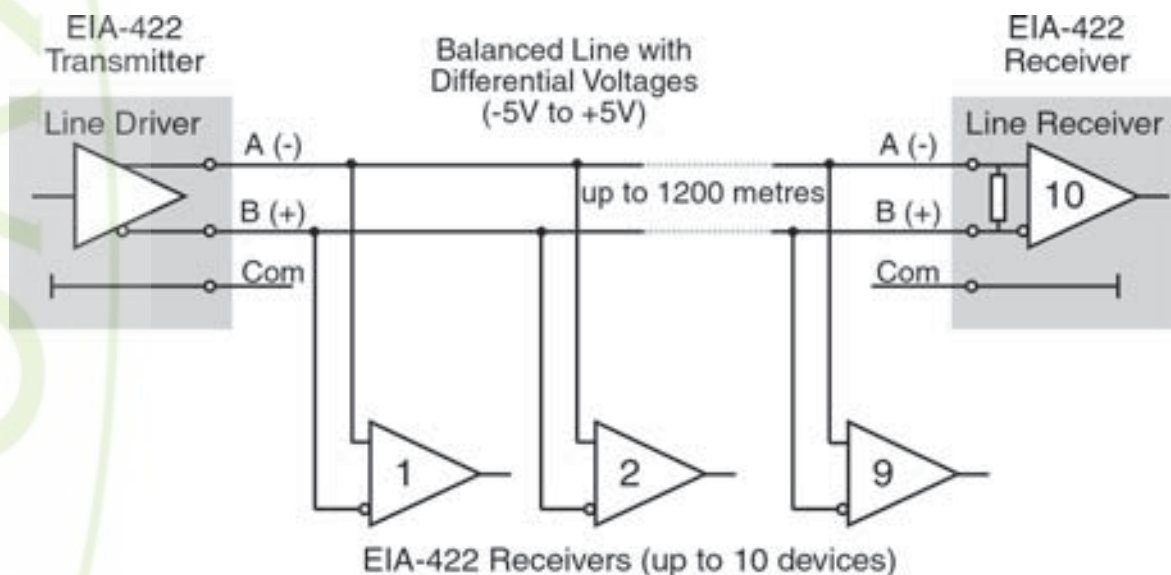
Figure 1.3 RS-422 Connection
