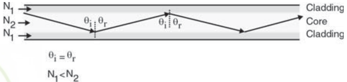
Figure 3.2 Light Ray Travelling Through an Optical Fiber
