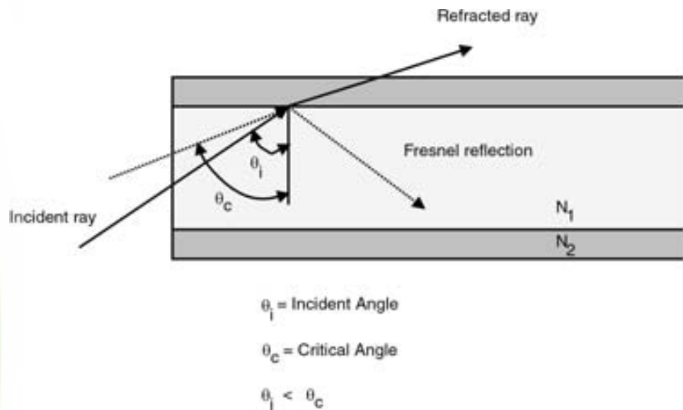
Figure 3.4 Fresnel Reflection
