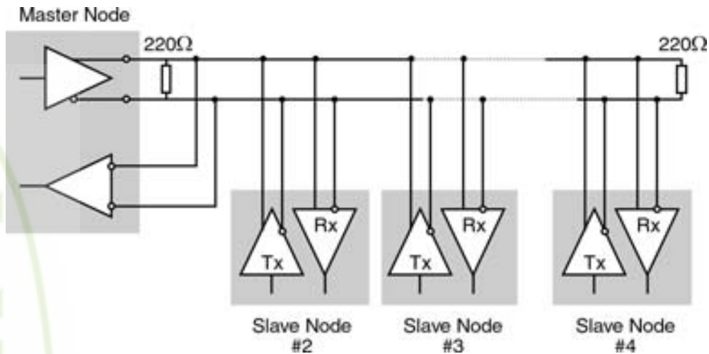
Figure 1.4 RS-485 Connection
