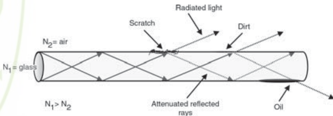
Figure 3.3 Problems Associated with a Glass Air Interface
