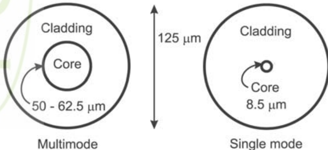
Figure 3.1 Optical Fiber Cross Sections
