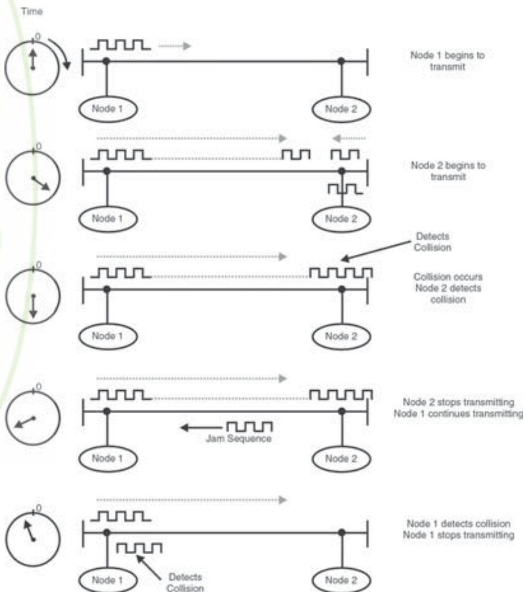
Figure 2.4 Operation of CSMA/CD
