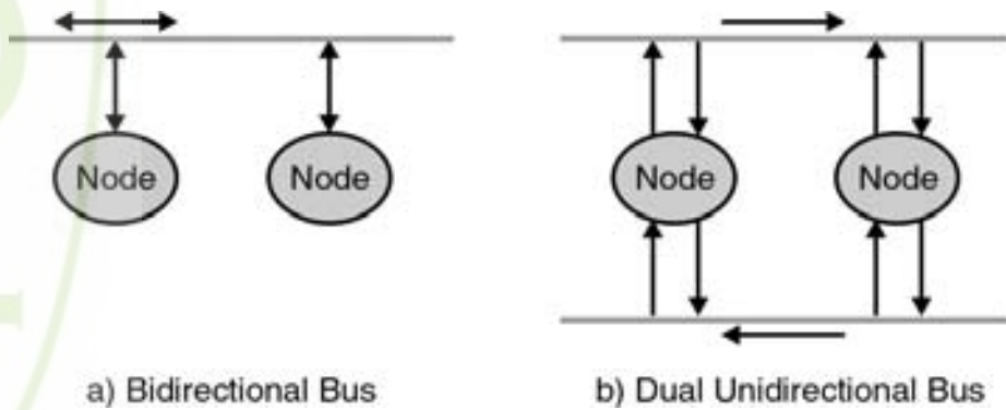
Figure 2.3 Examples of Bus Network Topology
